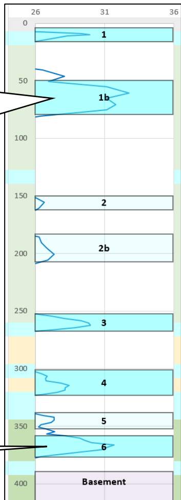
Extract of possible water-rich layers from Adrok's processing results
