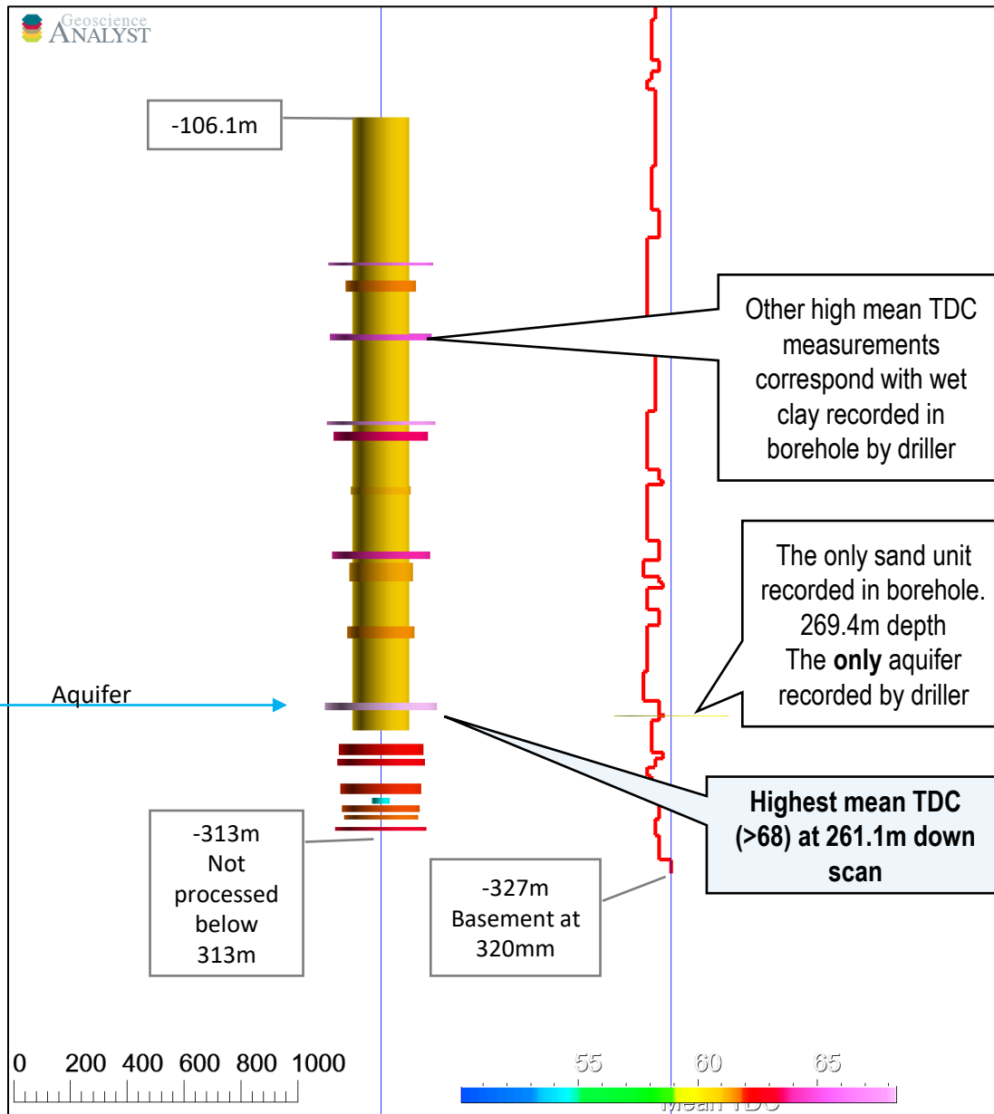
Screen capture from Geoscience Analyst 3D model showing ADR scan (left) and borehole log (right)
